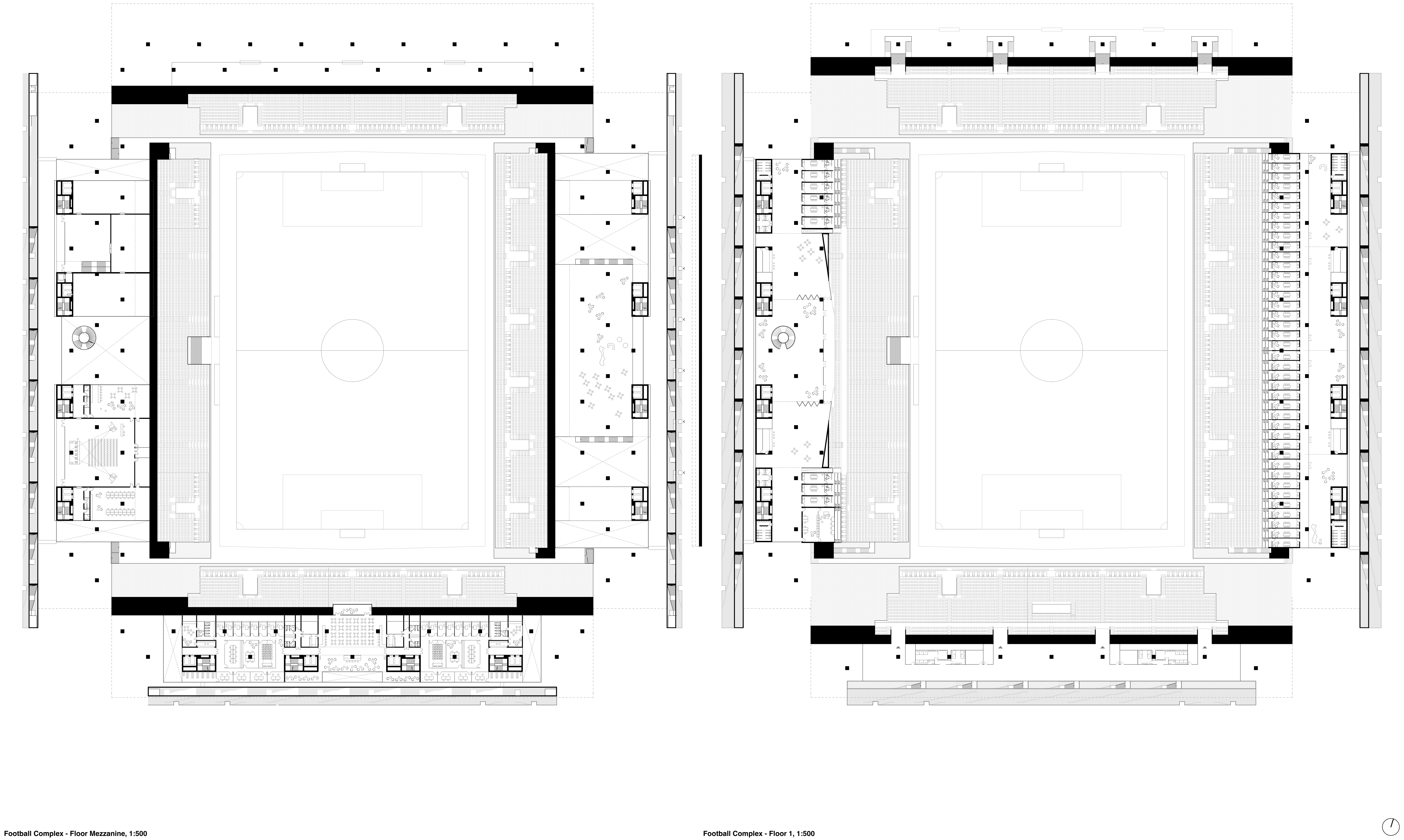
Football Complex - Floor Mezzanine, 1:500
