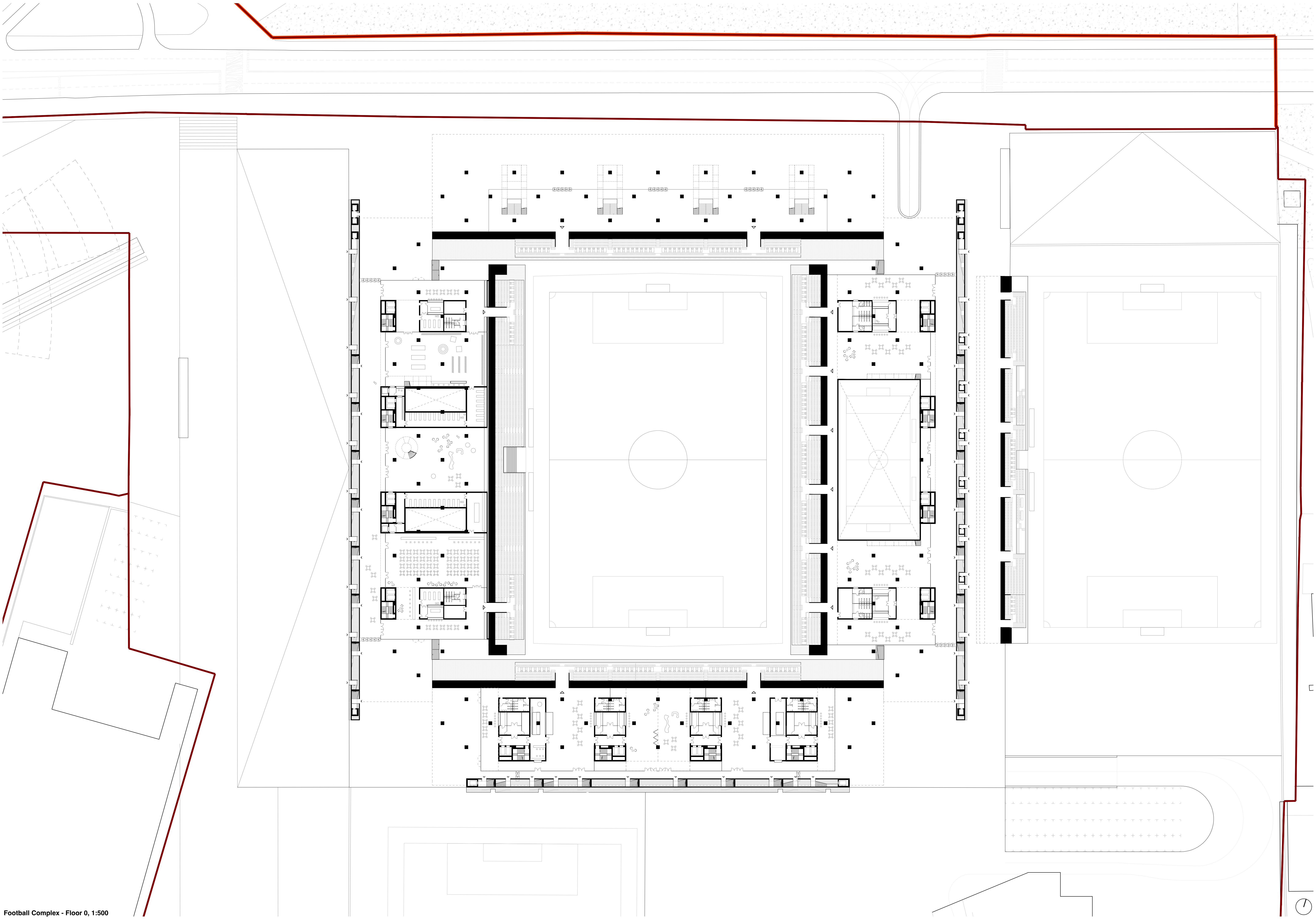
Football Complex - Floor 0, 1:500
