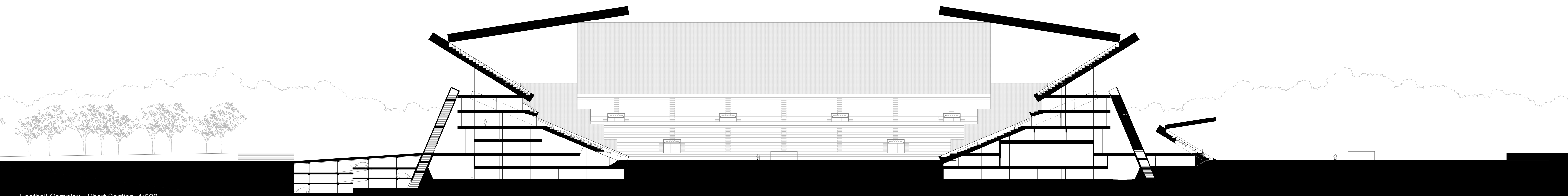
Football Complex - Short Section, 1:500
